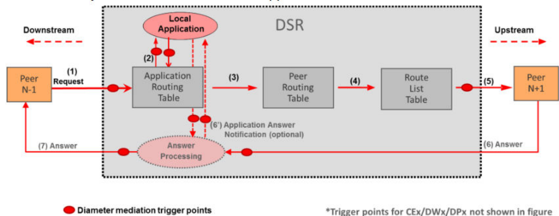
Figure 2-44 Mediation Trigger Points
